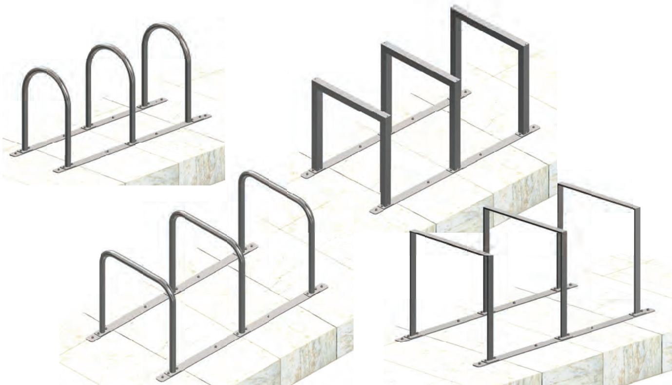
Bicycle parking rack - With guide rails for screwing on hoops height: 800mm, hoop spacing: 700mm. hot-dip galvanized
