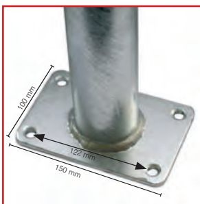
Bottom Plate
